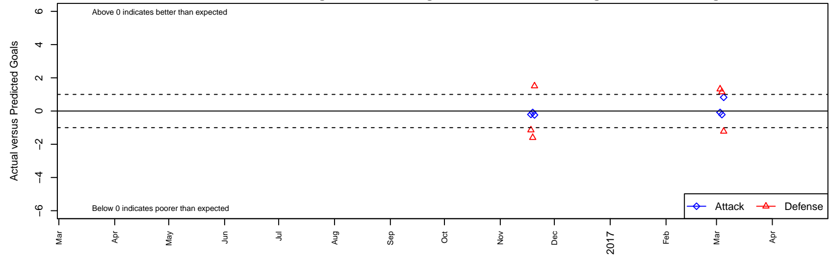
Las Vegas Neon Blue G02 Dots are actual minus expected GF (blue circles) and GA (red triangles). Blue line is smoothed change in attack strength. Red is smoothed change in defense strength.
